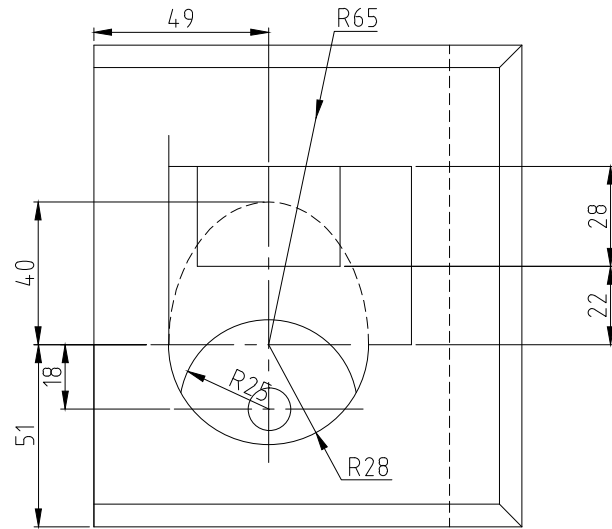
TOP SCALE 1/2
