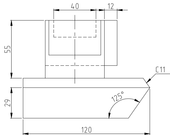
TOP SCALE 1/2
