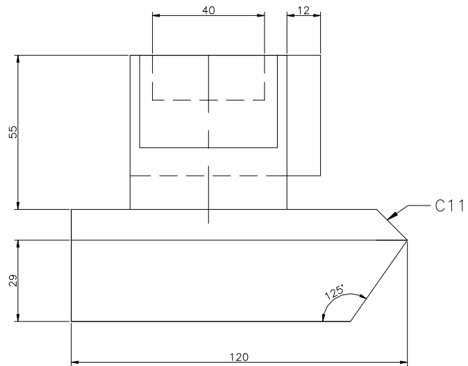
FRONT SCALE 1/2
