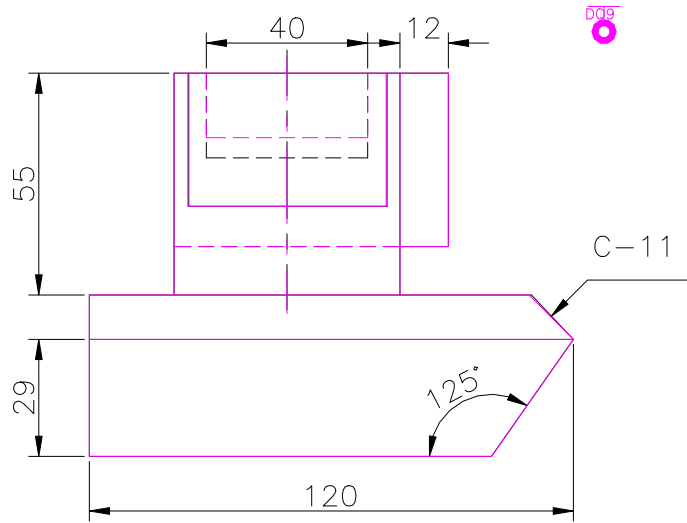
FRONT SCALE 1/2
