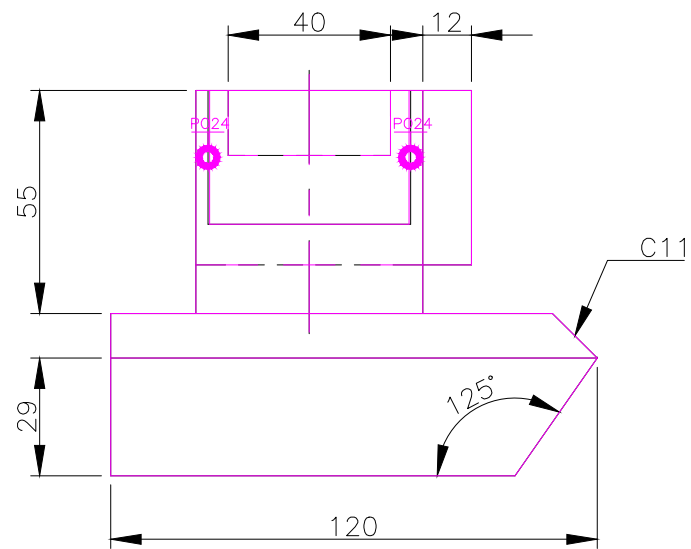
FRONT SCALE 1/2
