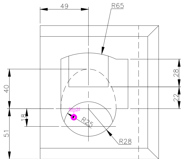
TOP SCALE 1/2
