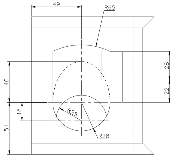
TOP SCALE 1/2
