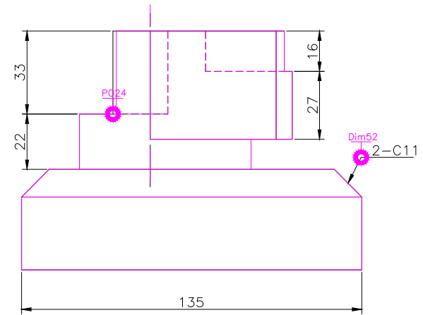
RIGHT SCALE 1/2
