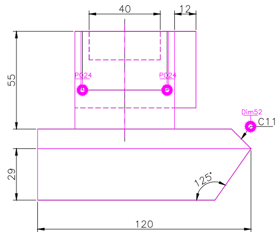
FRONT SCALE 1/2
