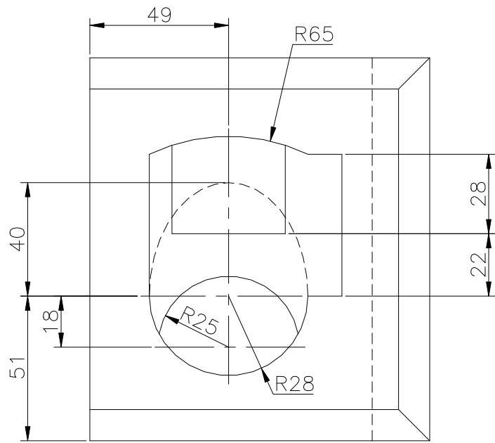
TOP SCALE 1/2
