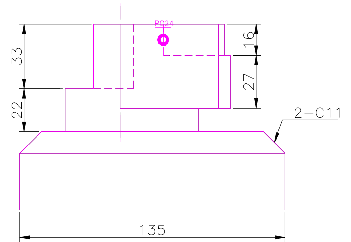
RIGHT SCALE 1/2
