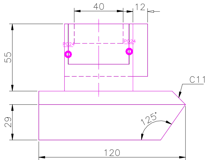
FRONT SCALE 1/2
