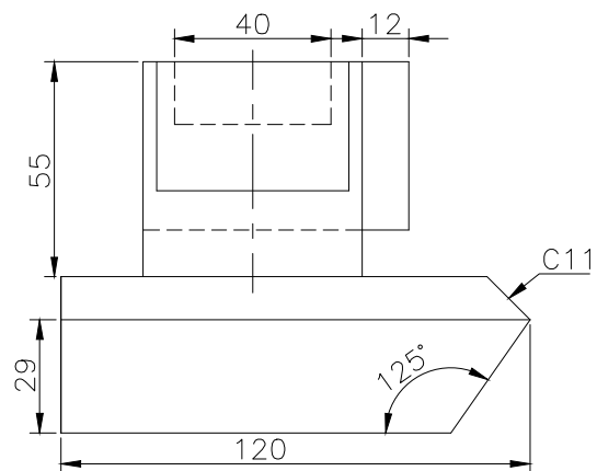
FRONT SCALE 1/2
