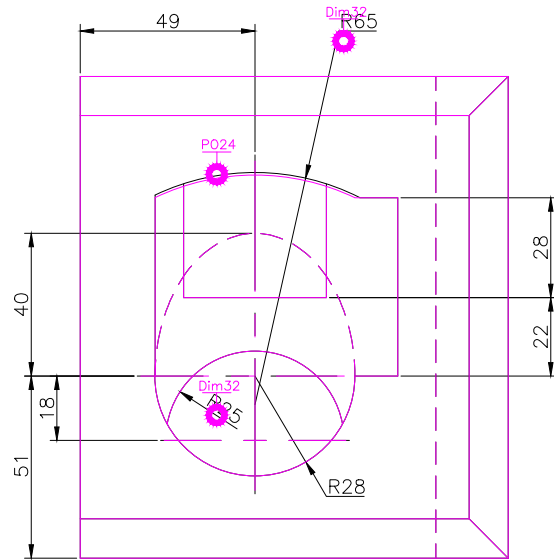
TOP SCALE 1/2
