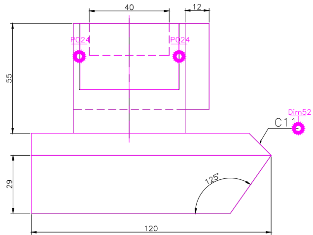
FRONT SCALE 1/2
