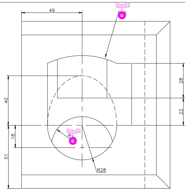
TOP SCALE 1/2
