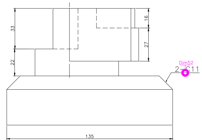
RIGHT SCALE 1/2
