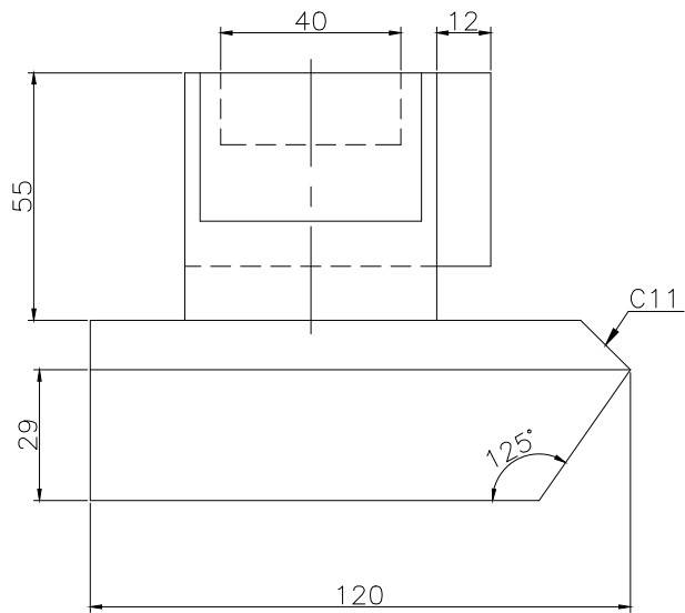
FRONT Scale 2/1
