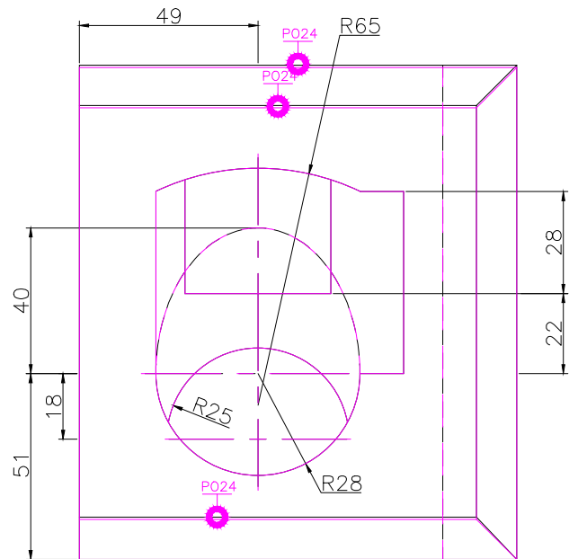
Top Scale 2/1
