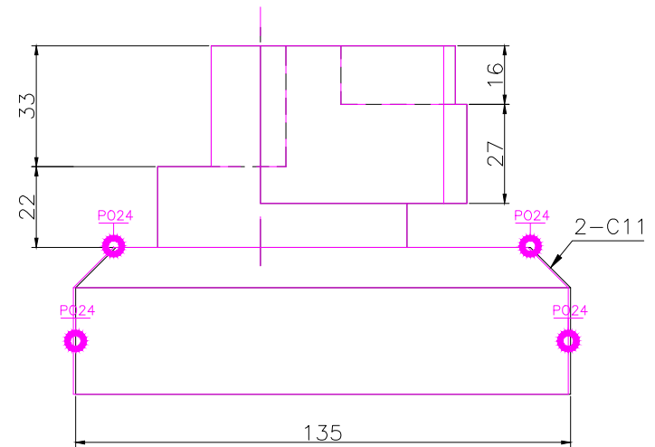
Top Scale 2/1
