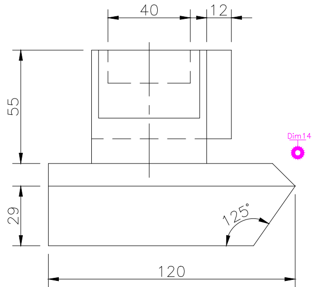
FRONT SCALE 1/2
