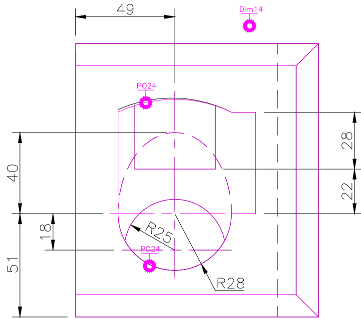
TOP SCALE 1/2
