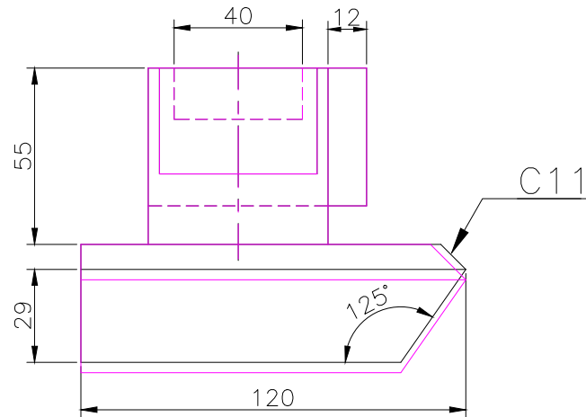
FRONT SCALE 1/2
