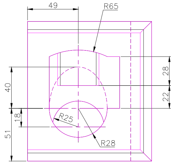
TOP SCALE 1/2
