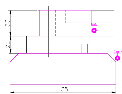
RIGHT SCALE 1/2
