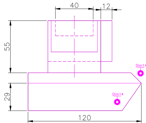
FRONT SCALE 1/2
