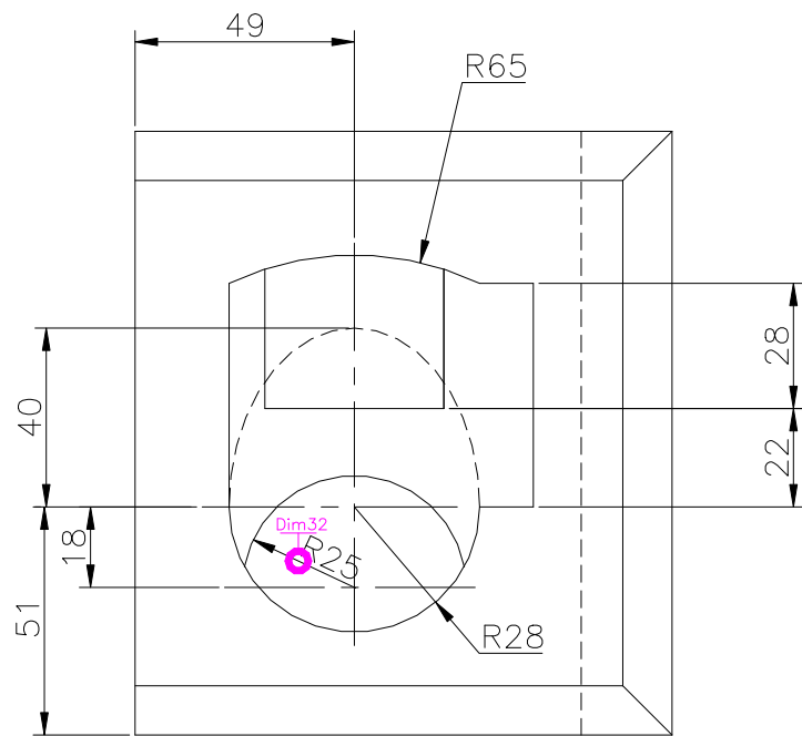
TOP SCALE 1/2
