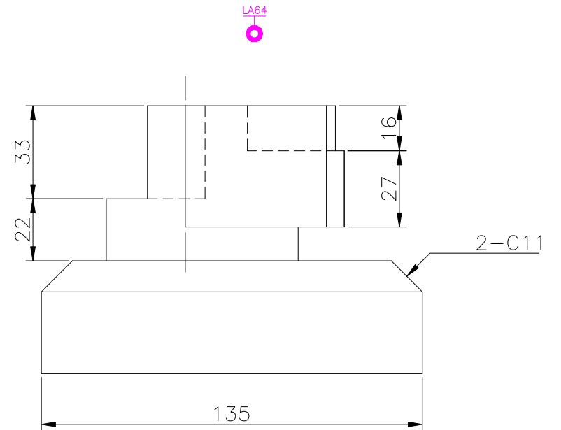
RIGHT SCALE 1/2
