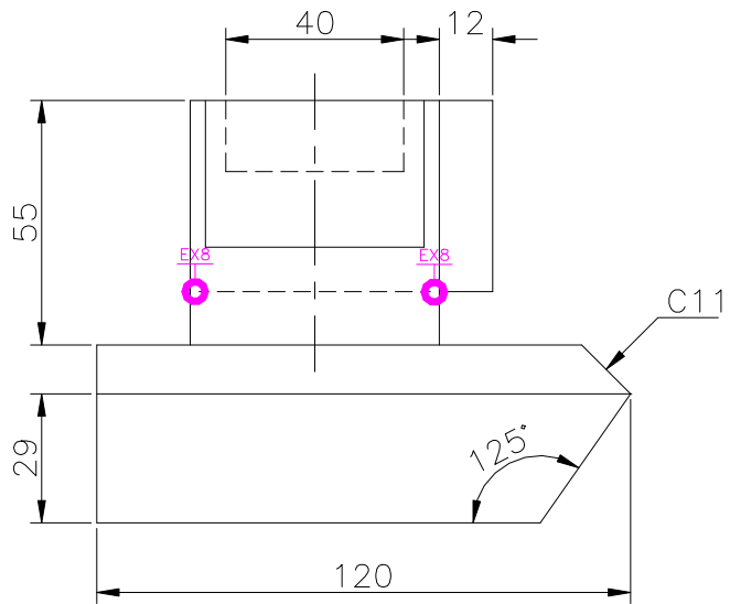
FRONT SCALE 1/2
