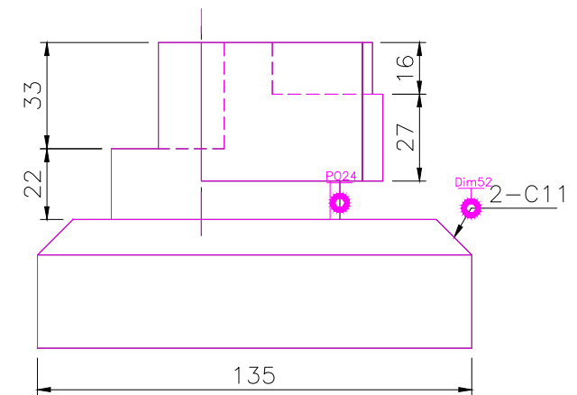
RIGHT SCALE 1/2
