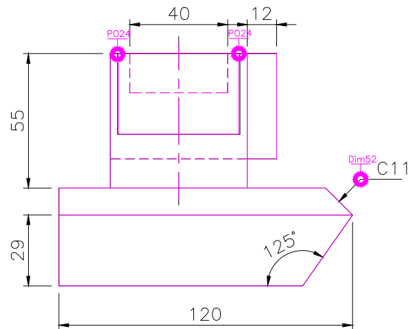
FRONT SCALE 1/2
