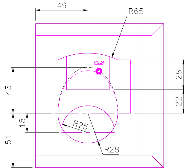
TOP SCALE 1/2
