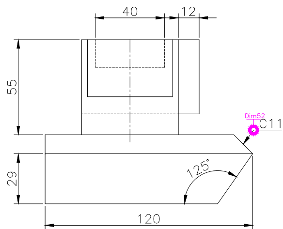
FRONT SCALE 1/2
