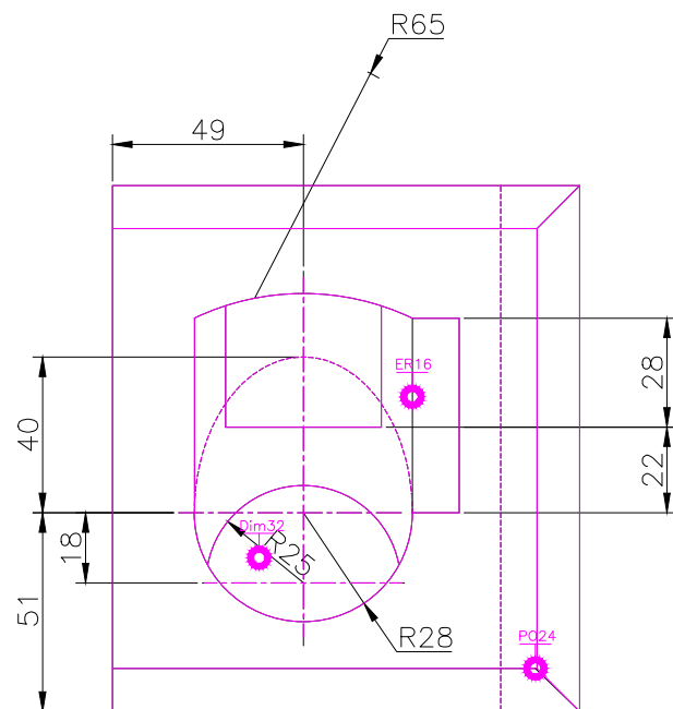
TOP SCALE 1/2
