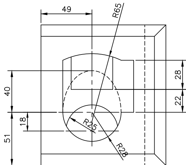
TOP SCALE 1/2
