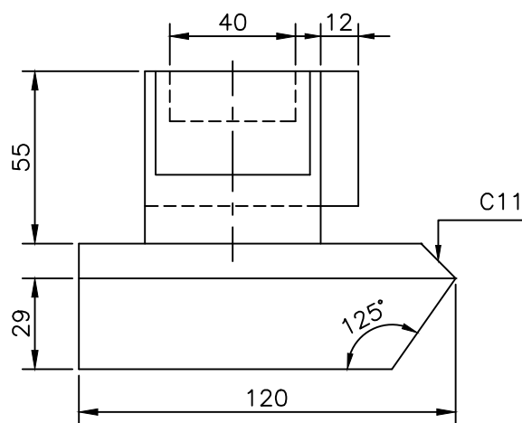
FRONT SCALE 1/2
