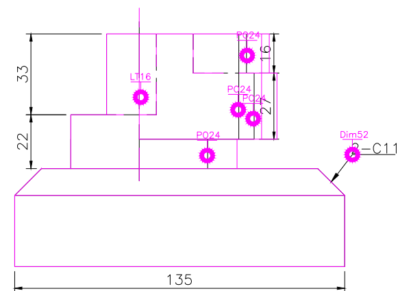
RIGHT SCALE 1/2
