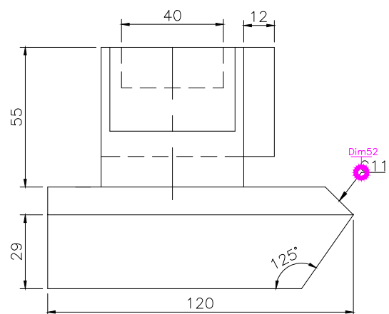
FRONT SCALE 1/2
