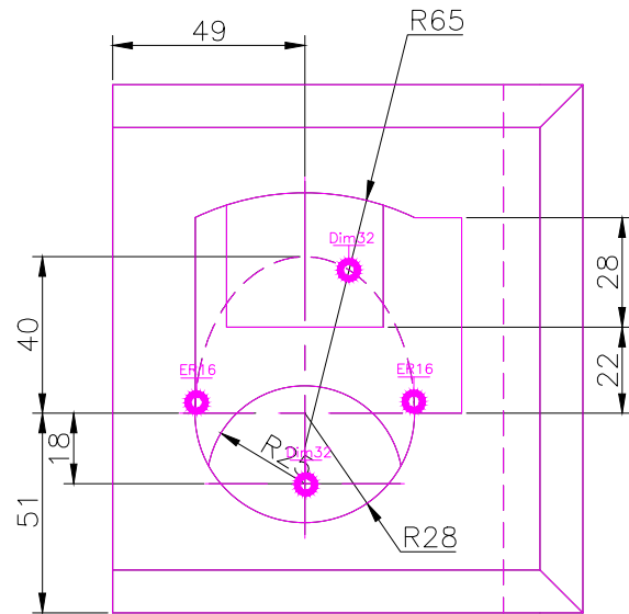
TOP SCALE 1/2
