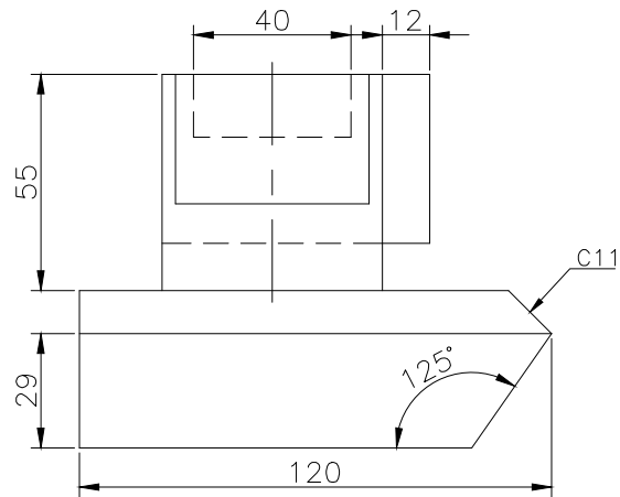
FRONT SCALE 1/2
