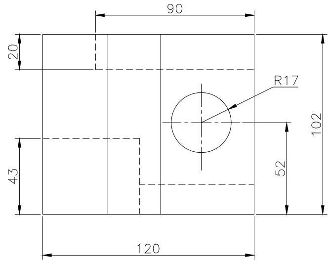
RIGHT SCALE 1/2
