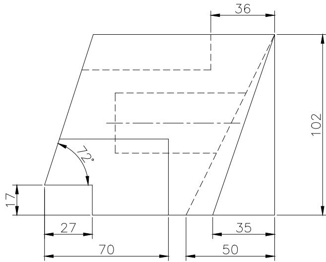
FRONT SCALE 1/2
