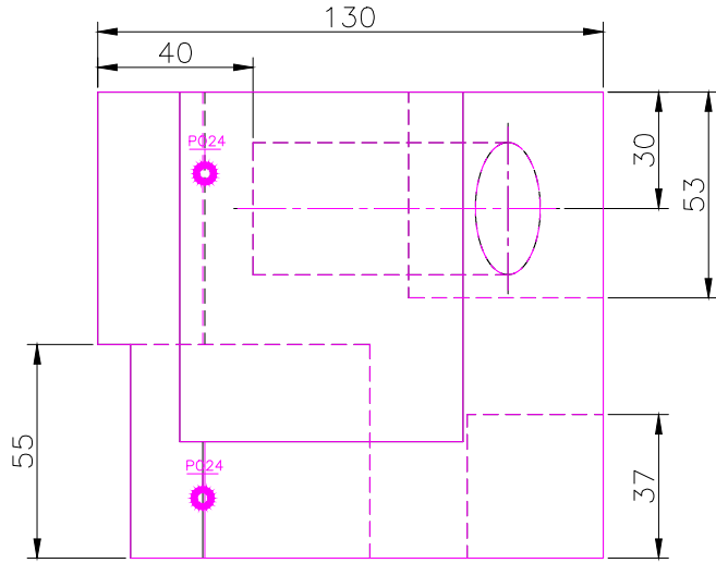
TOP SCALE 1/2
