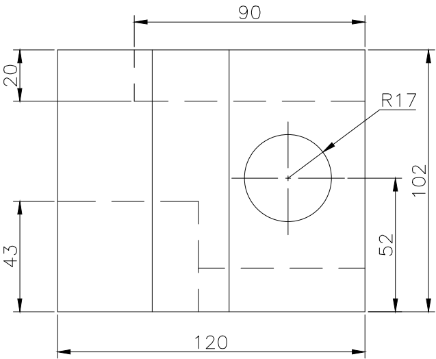
RIGHT SCALE 1/2
