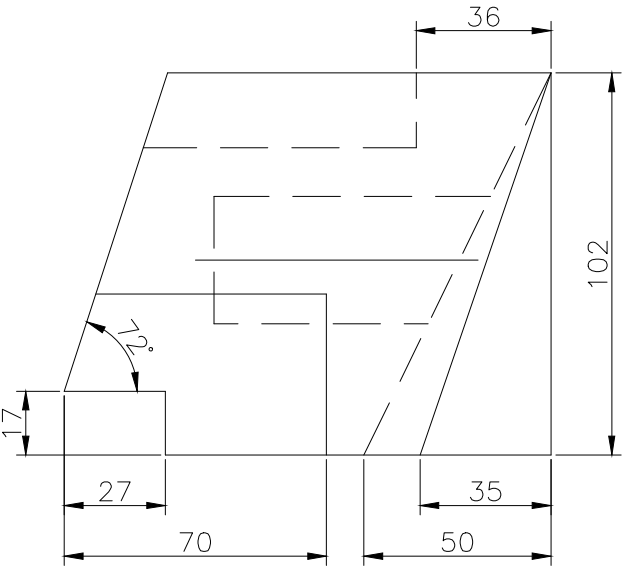
FRONT SCALE 1/2
