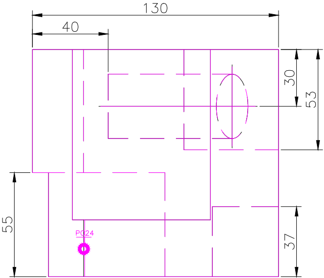
TOP SCALE 1/2
