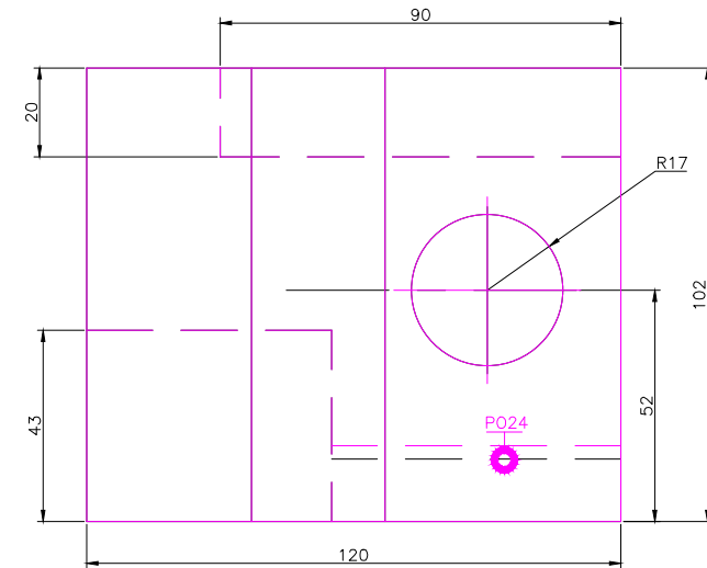
RIGHT SCALE 1/2
