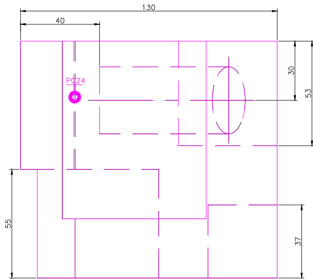
TOP SCALE 1/2
