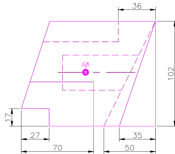
FRONT SCALE 1/2
