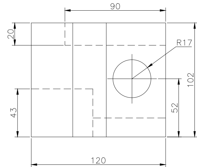
RIGHT SCALE 1/2
