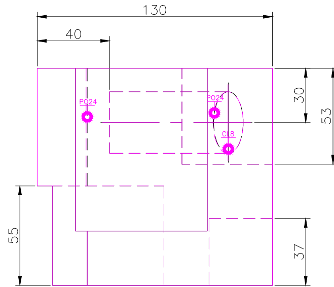
TOP SCALE 1/2
