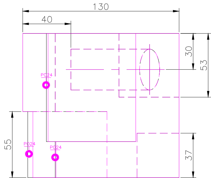
TOP SCALE 1/2
