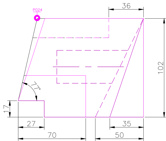
FRONT SCALE 1/2
