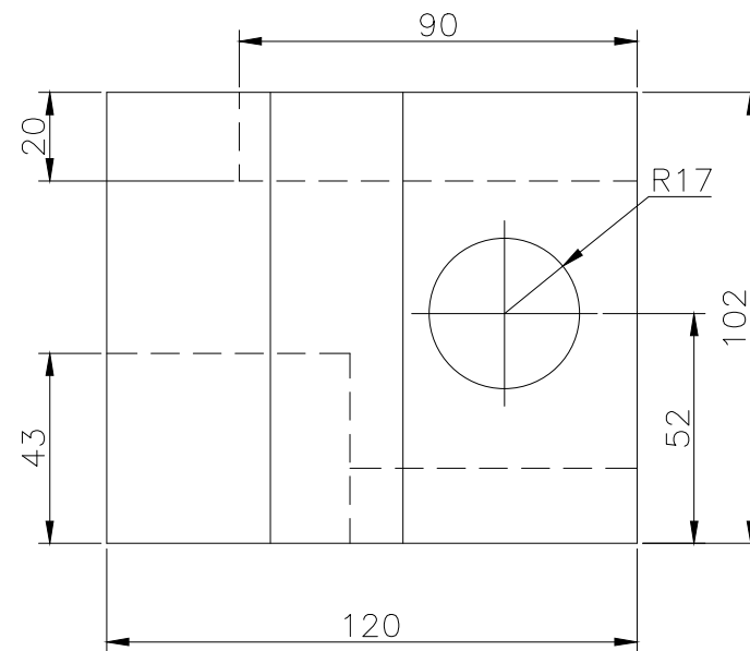
RIGHT SCALE 1/2
