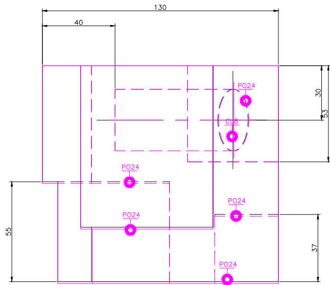
TOP SCALE 1/2
