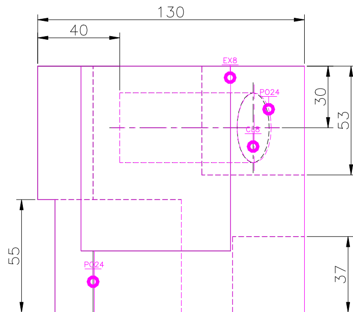
TOP SCALE 1/2
