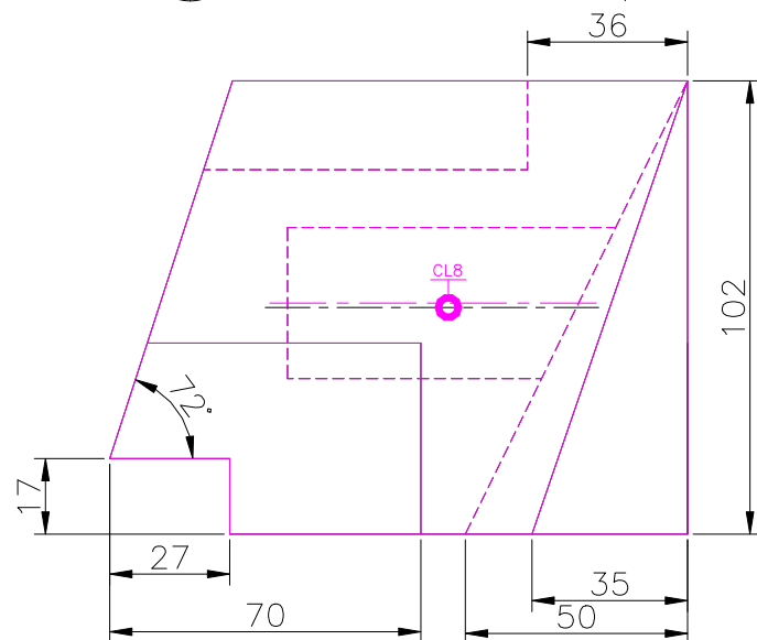
FROUNT SCALE 1/2
