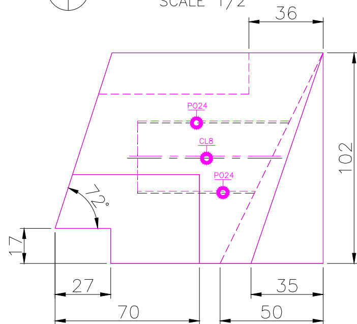
FRONT SCALE 1/2
