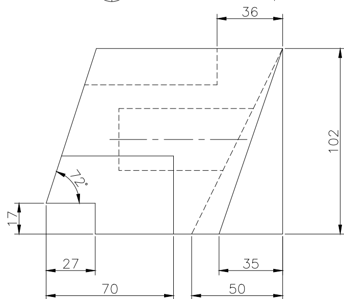
FRONT SCALE 1/2
