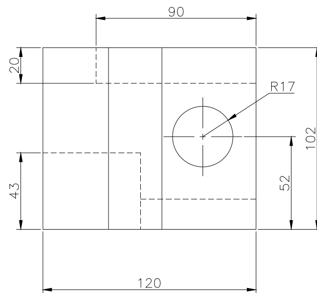
RIGHT SCALE 1/2
