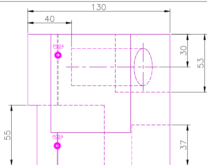
TOP SCALE 1/2
