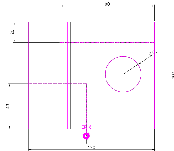
RIGHT scale 1/2
