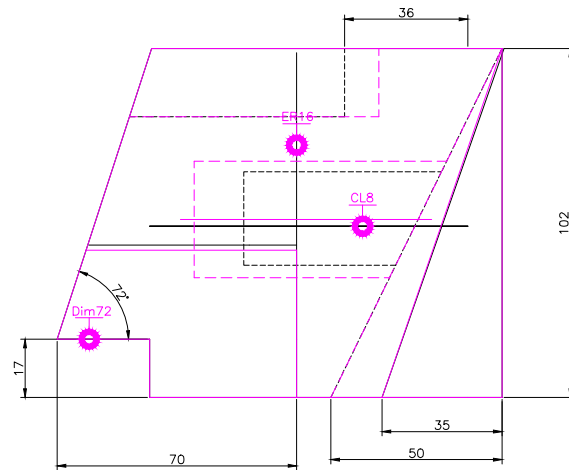
FRONT scale 1/2
