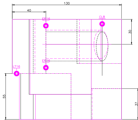
TOP scale 1/2
