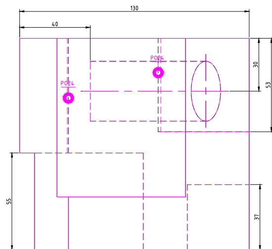
TOP SCALE 1/2
