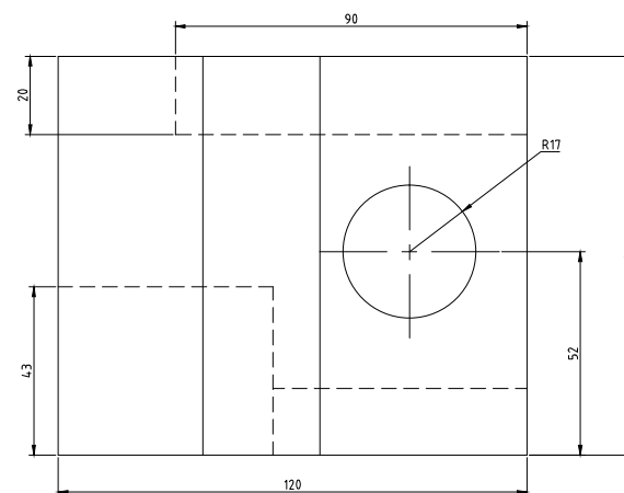
RIGHT SCALE 1/2
