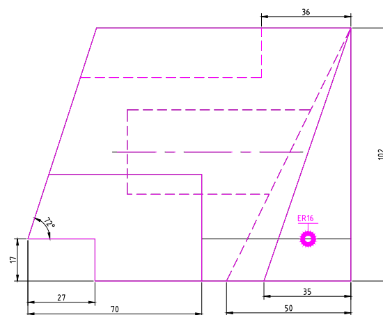
FRONT SCALE 1/2
