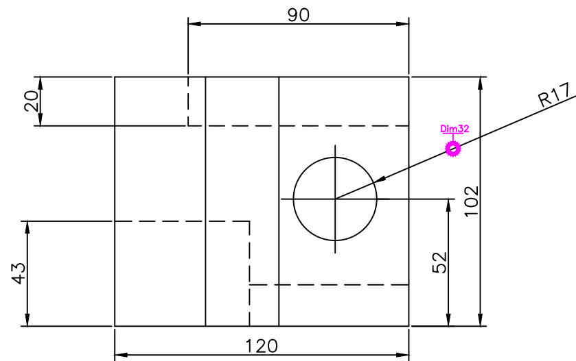
RIGHT SCALE 1/2
