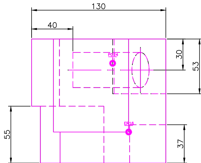
TOP SCALE 1/2
