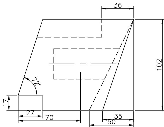
FRONT SCALE 1/2
