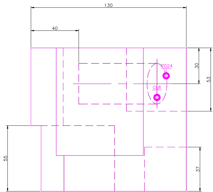
TOP SCALE 1/2
