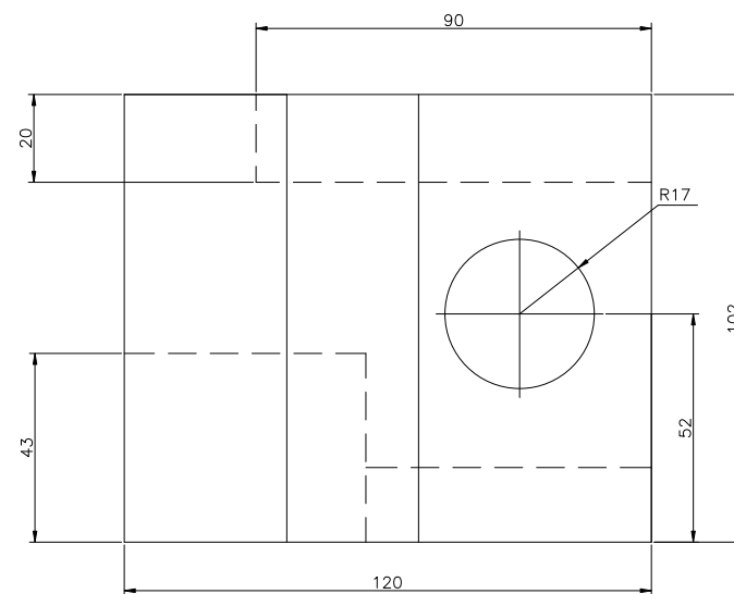
RIGHT SCALE 1/2
