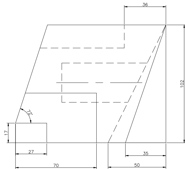
FRONT SCALE 1/2
