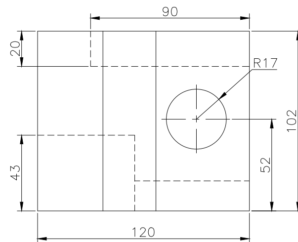
RIGHT SCALE 1/2
