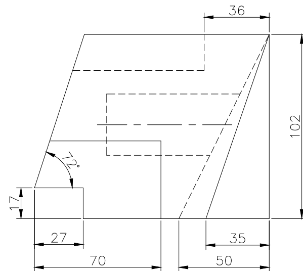
FRONT SCALE 1/2
