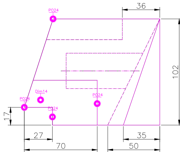
FRONT SCALE 1/2
