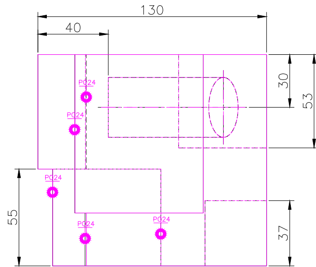
TOP SCALE 1/2
