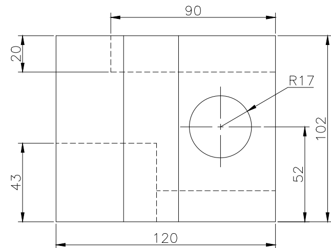
RIGHT SCALE 1/2
