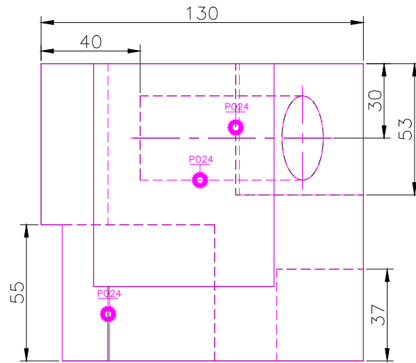
TOP SCALE 1/2
