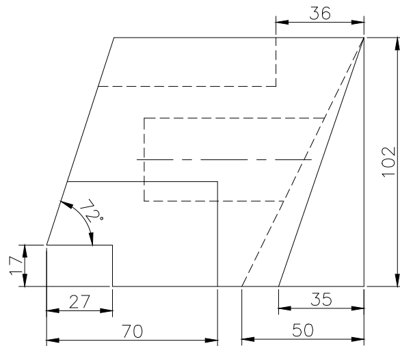
FRONT SCALE 1/2
