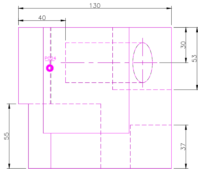
TOP SCALE 1/2
