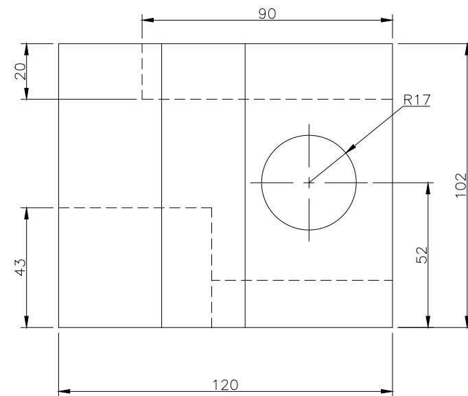
RIGHT SCALE 1/2
