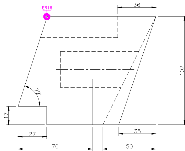
FRONT SCALE 1/2
