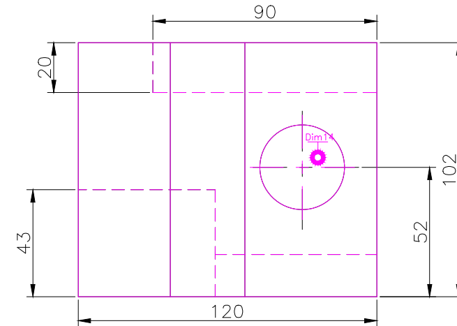
RIGHT SCALE 1/2
