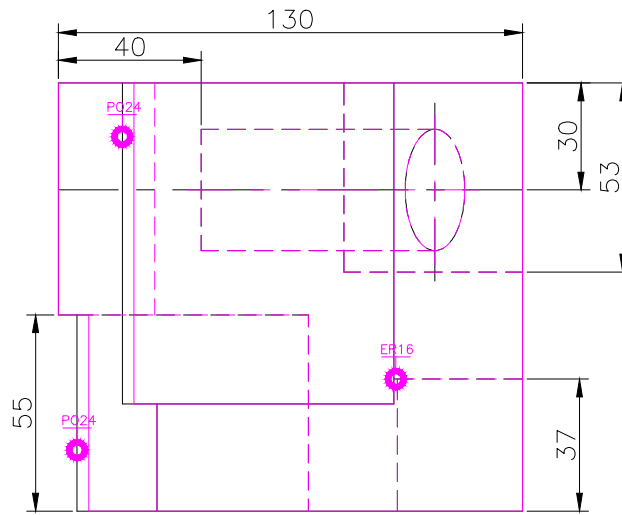
TOP SCALE 1/2
