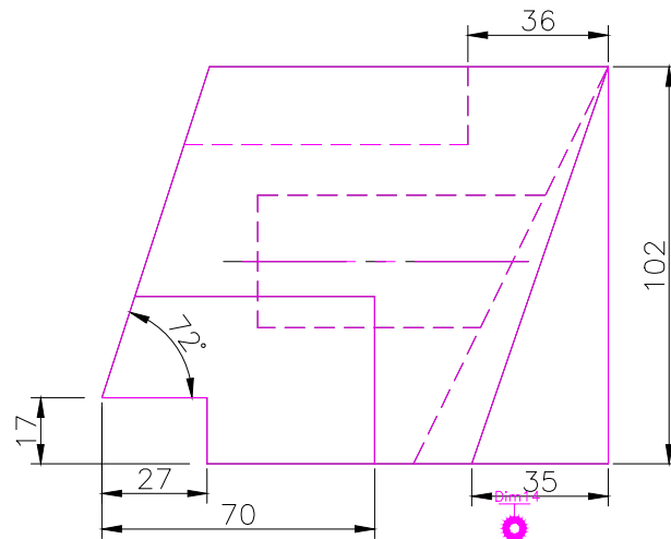
FRONT SCALE 1/2
