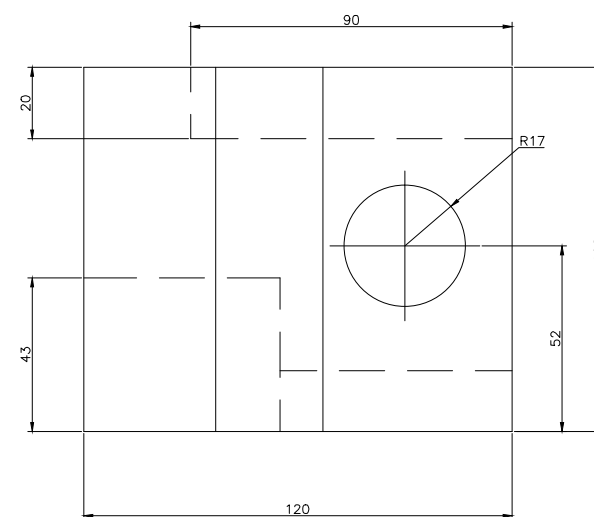
RIGHT SCALE 1/2
