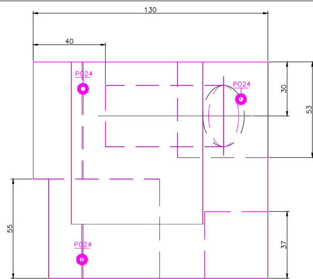
TOP SCALE 1/2
