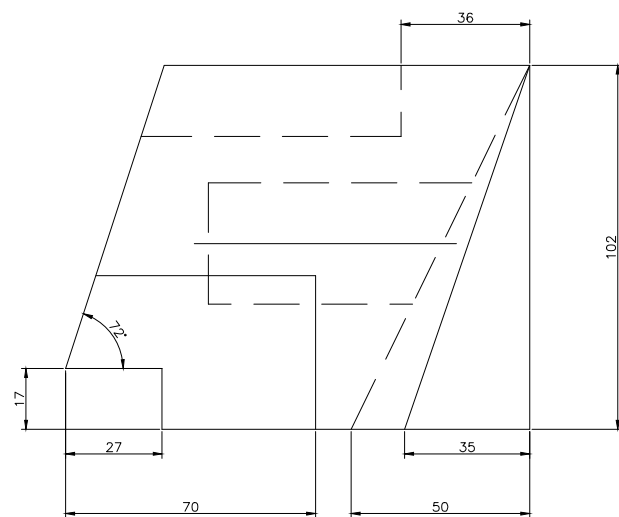
FRONT SCALE 1/2
