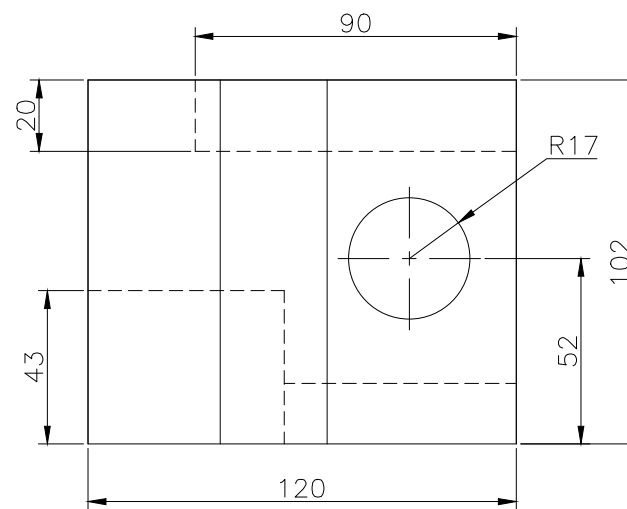
RIGHT SCALE 1/2
