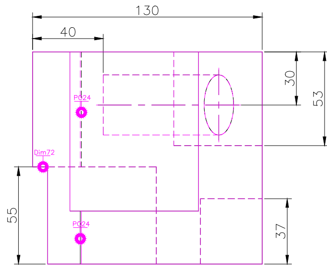
TOP SCALE 1/2
