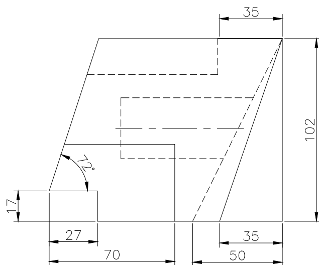
FRONT SCALE 1/2
