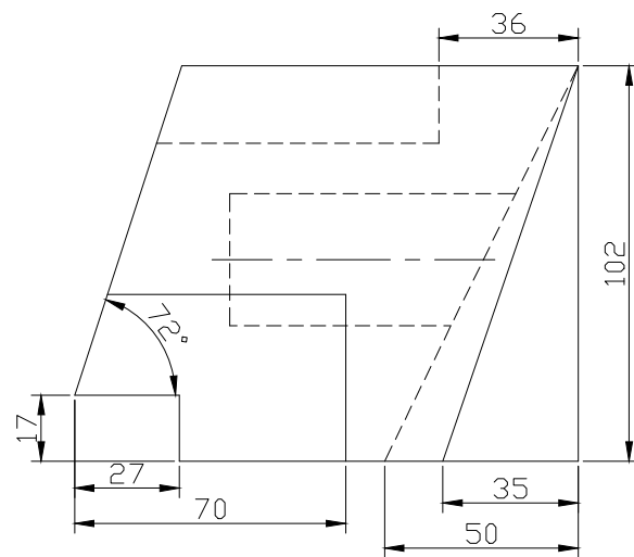
FRONT SCALE 1/2
