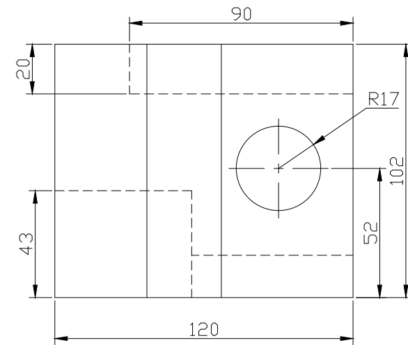
RIGHT SCALE 1/2
