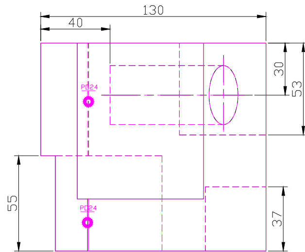
TOP SCALE 1/2
