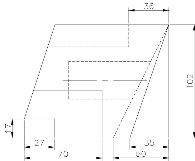
FRONT SCALE 1/2
