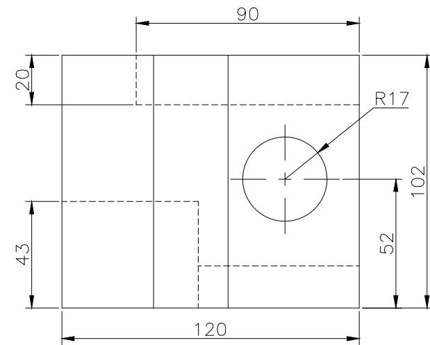
RIGHT SCALE 1/2
