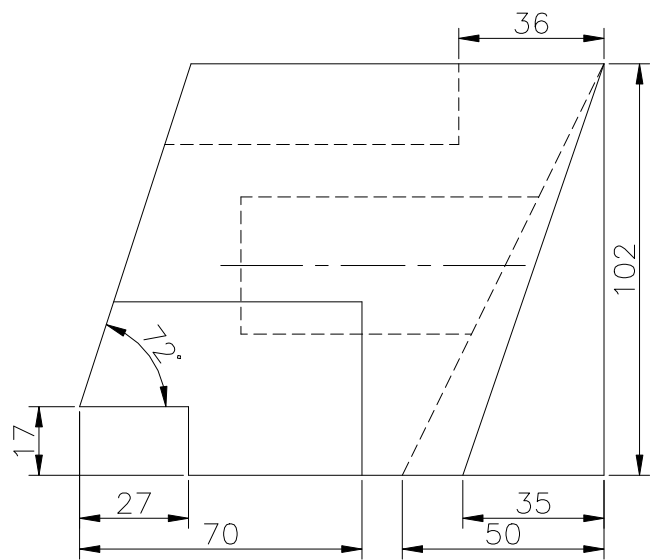
FRONT SCALE 1/2
