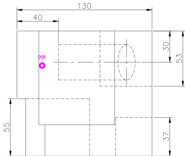
TOP SCALE 1/2
