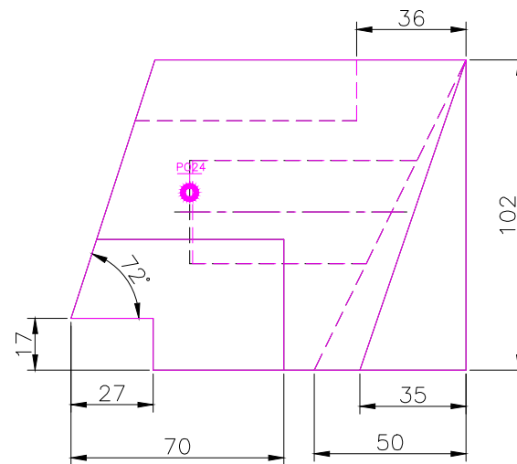
FRONT SCALE 1/2
