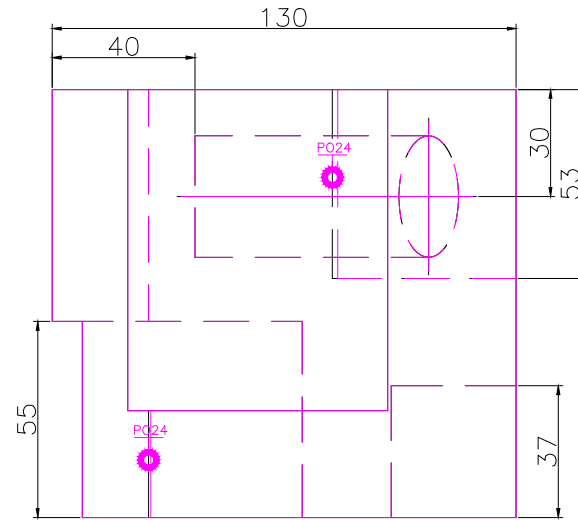
TOP SCALE 1/2
