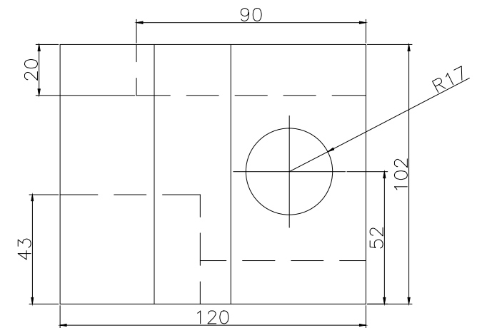
RIGHT SCALE 1/2
