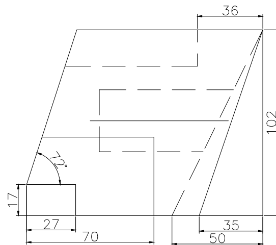
FRONT SCALE 1/2
