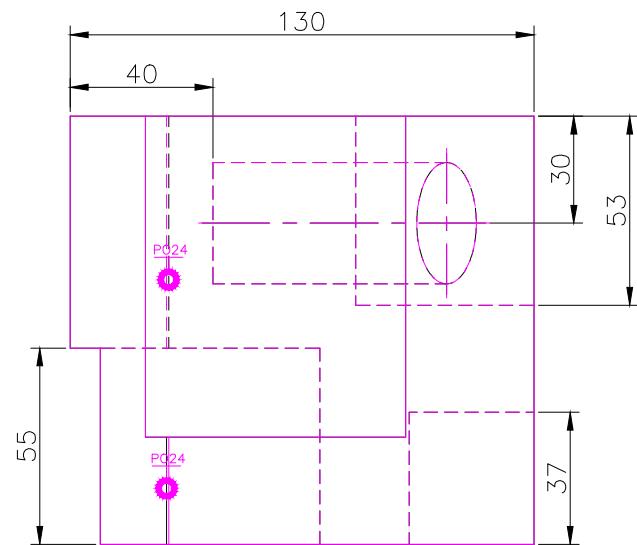
TOP SCALE 1/2
