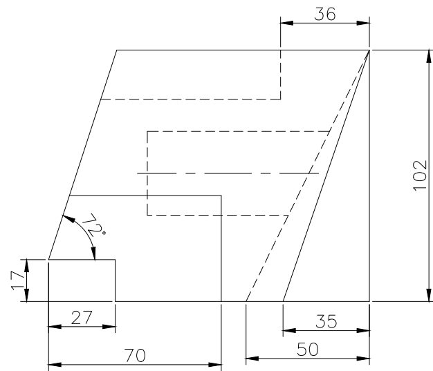
FRONT SCALE 1/2
