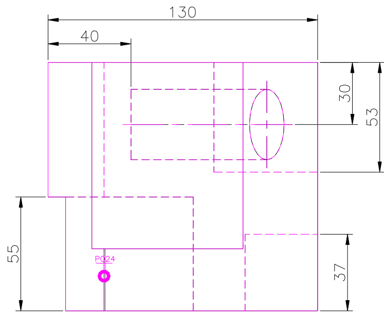
TOP SCALE 1/2
