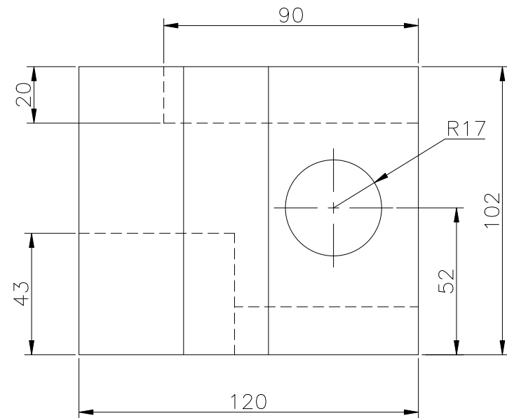
RIGHT SCALE 1/2
