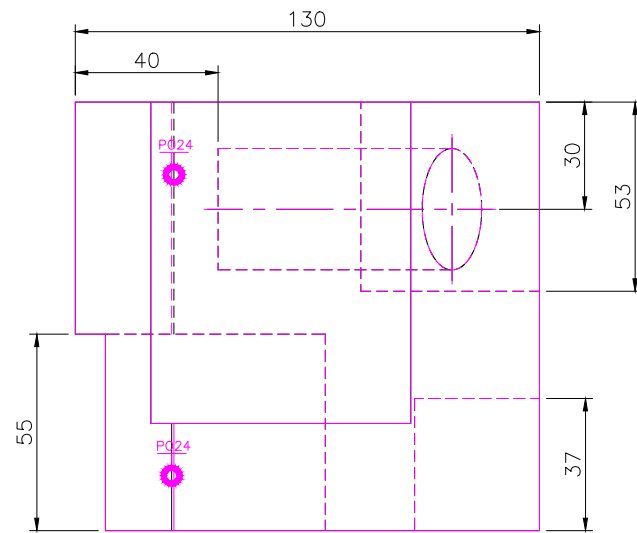
TOP SCALE 1/2
