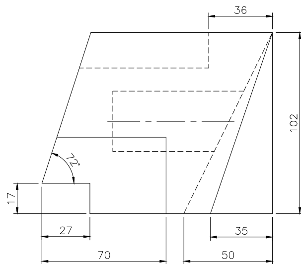
FRONT SCALE 1/2
