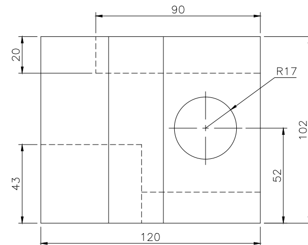
RIGHT SCALE 1/2
