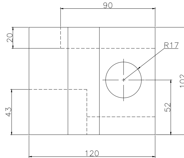
RIGHT SCALE 1/2
