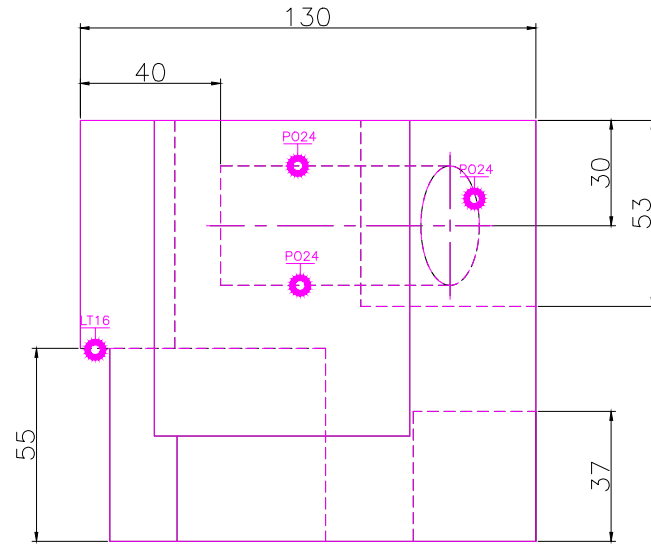
TOP SCALE 1/2
