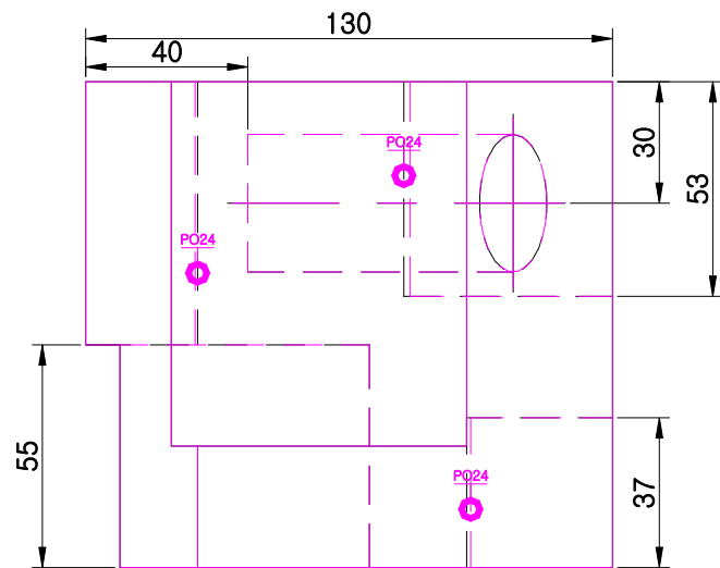
TOP SCALE 1/2
