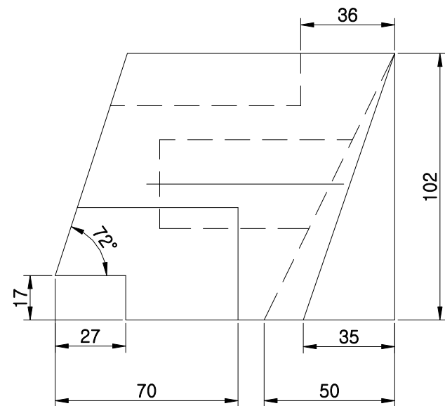
FRONT SCALE 1/2
