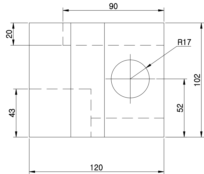
RIGHT SCALE 1/2
