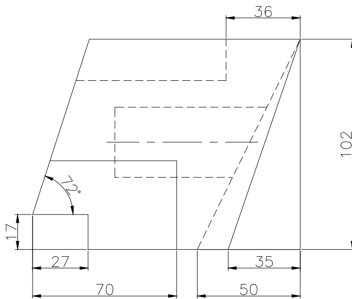
FRONT SCALE 1/2
