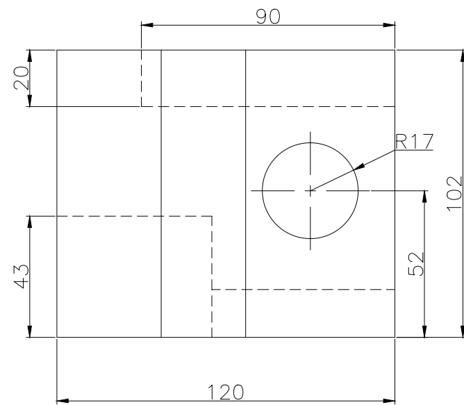
RIGHT SCALE 1/2
